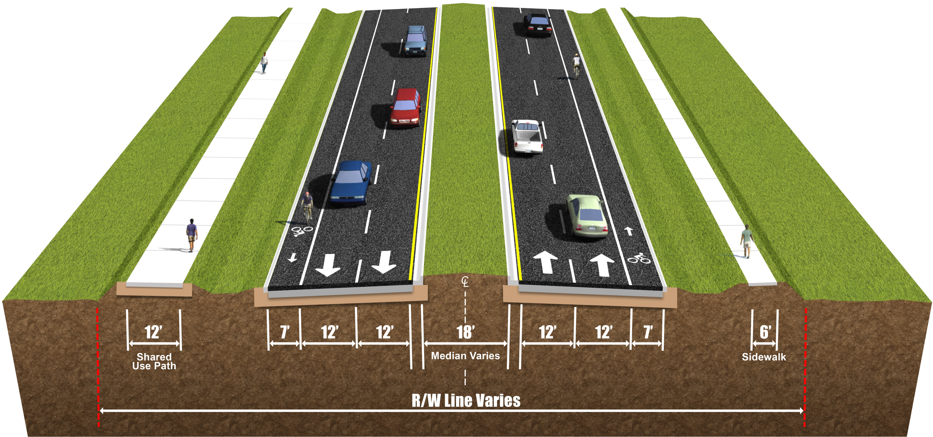
INTERIM — 4-LANE TYPICAL SECTION
