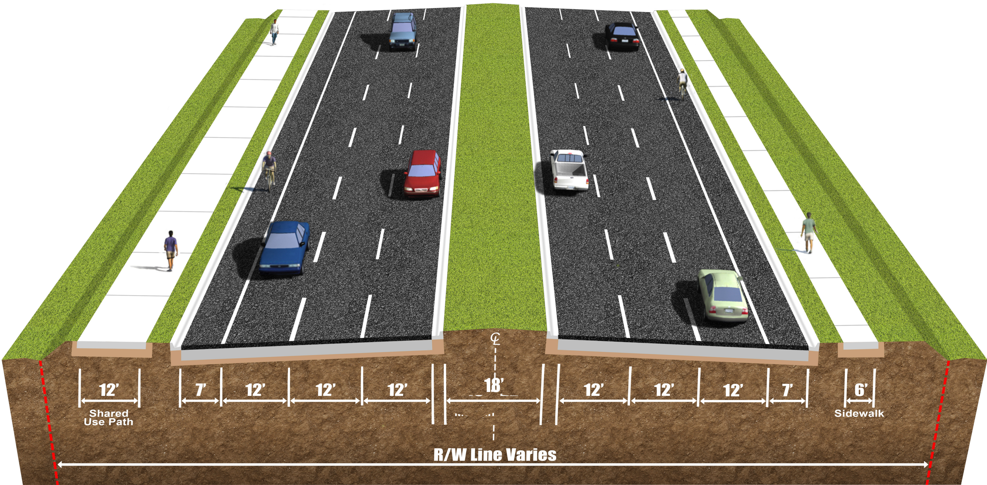
ULTIMATE — 6-LANE TYPICAL SECTION
